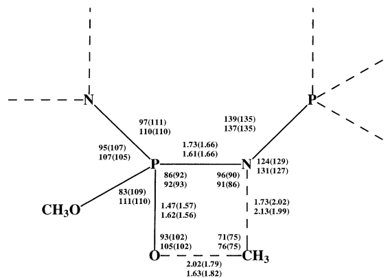
Fig. 1 Key structural features of the aa \rightarrow aa\beta and aa \rightarrow aaa transition structures. The important geometric features for the aa \rightarrow aaa transition structure are shown above those for the aa \rightarrow aa\beta transition structure. The corresponding features for the equilibrium structure are in parentheses. The key feature is that the key phosphorus atom has a more tetrahedral structure in the aa \rightarrow aa\beta transition structure (bond lengths in Å, angles in ^\circ )
